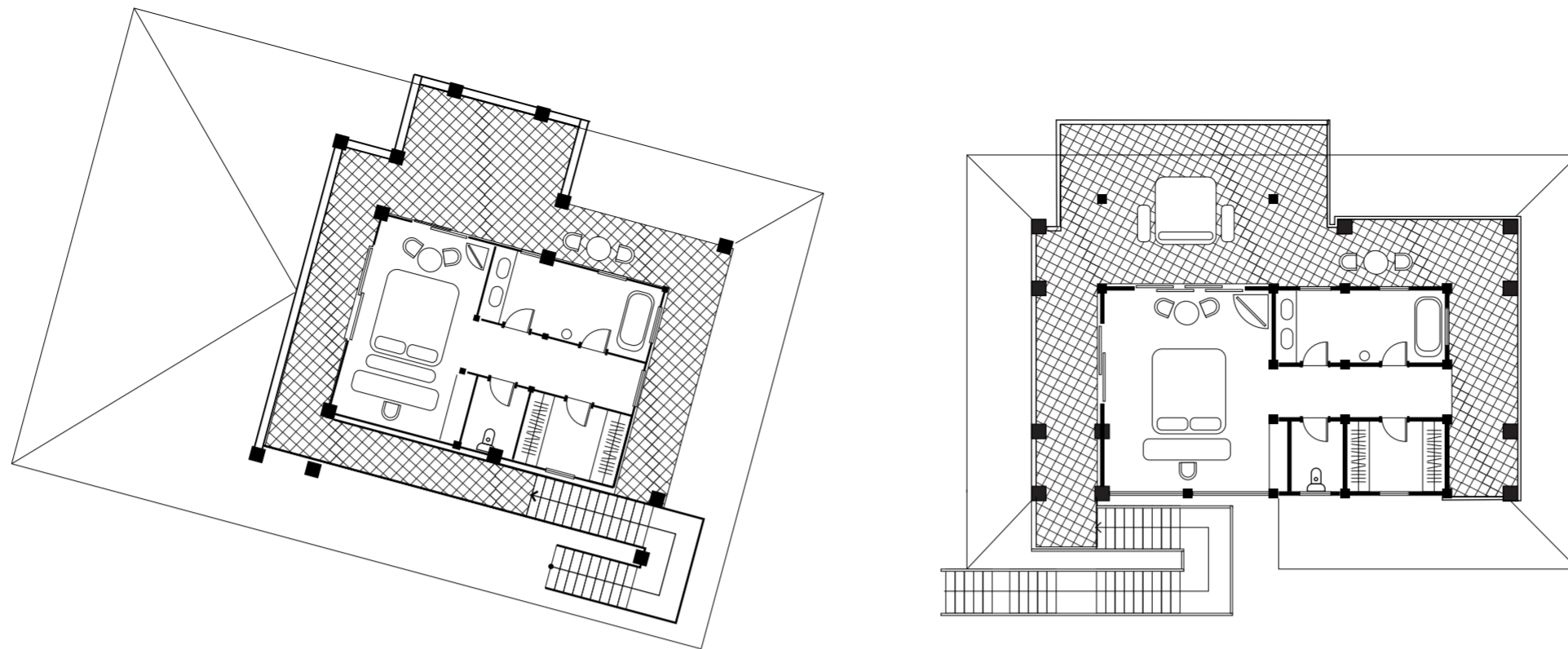
UPPER LEVEL
